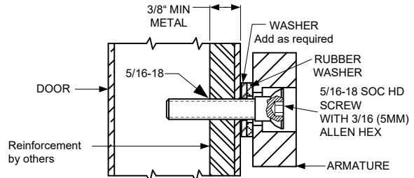
FIG. 2C REINFORCED DOOR
