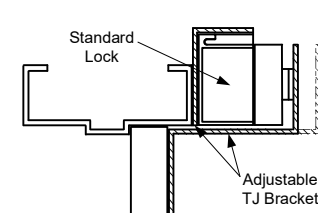
FIG. 1D Top Jamb Installation
